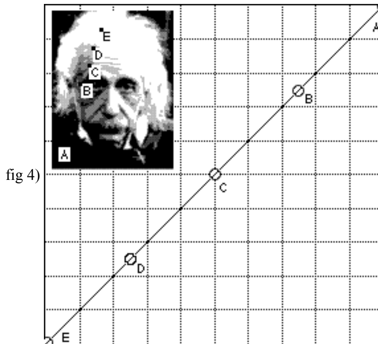
Clicking on shades with the eyedropper and observing the corresponding point in the Arbitrary Map
